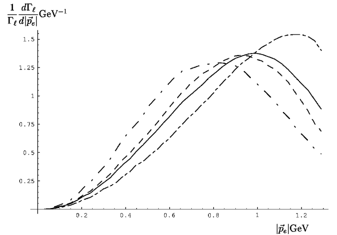
FIG. 4. The energy spectrum of the charged lepton for the decays B_c \rightarrow \chi_c + \tau + \nu_\tau , where the solid line is the result of h_c[1P_1] state, the dotted-blank-dashed line is of \chi_c[3P_0] , the dashed line is of \chi_c[3P_1] , and the dotted-dashed line is \chi_c[3P_2] .
