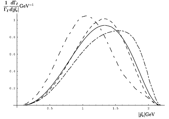
FIG. 3. The energy spectrum of the charged lepton for the decays B_c \rightarrow \chi_c + e(\mu) + \nu , where the solid line is the result of the h_c[1P_1] state, the dotted-blank-dashed line is of \chi_c[3P_0] , the dashed line is of \chi_c[3P_1] , and the dotted-dashed line is \chi_c[3P_2] .
